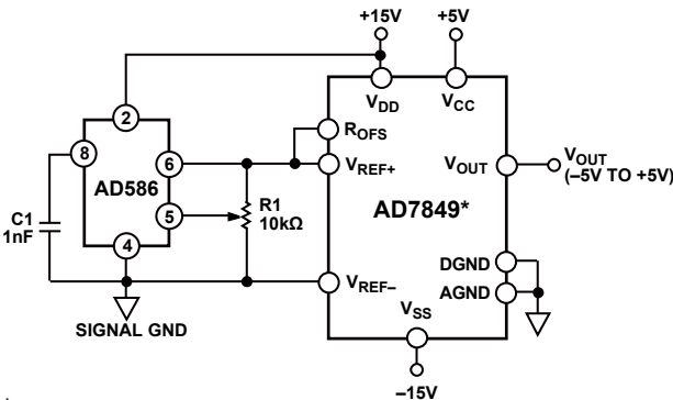
*ADDITIONAL PINS OMITTED FOR CLARITY. Figure 23. Generating a \pm 5 \text{ V} Output Range from a Single +5 V
